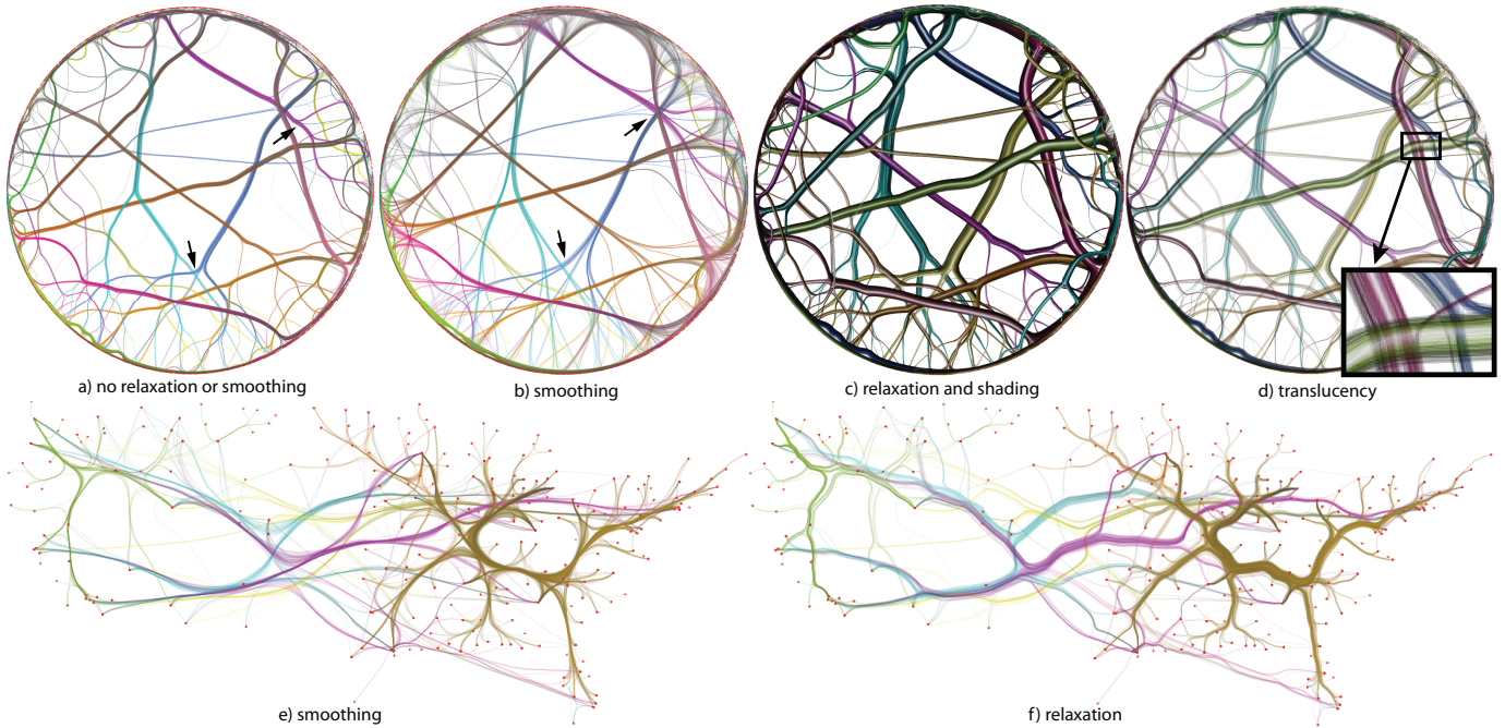
Fig. 5. Layout postprocessing. Edge smoothing (a vs b, Fig. 7 j vs e). Edge relaxation (Fig. 7 j vs f). Cushion shading (c), half-transparent detail (d)
