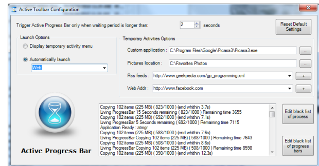
Figure 2: The Configuration window of the prototype.
